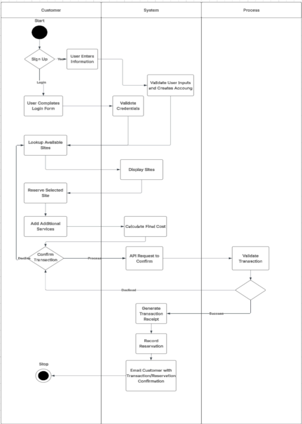
Activity Diagram:
